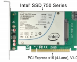
PCI Express x16 (4-Lane), V4.0
